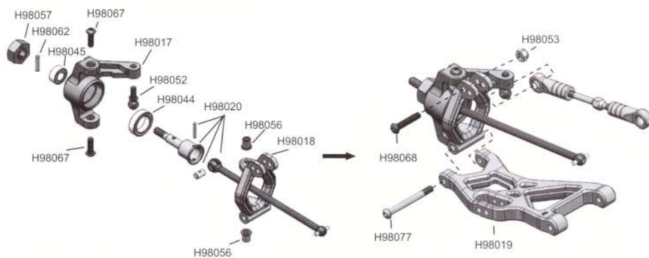
7. Suspension(2)
