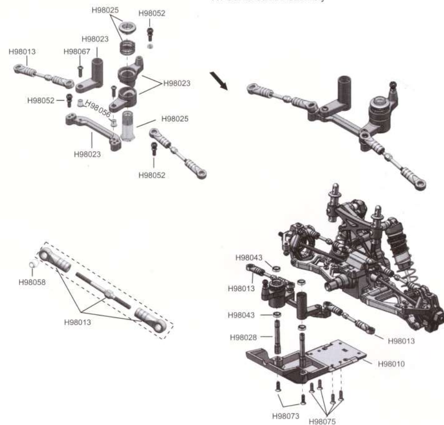
11. Servo Save Assembly
