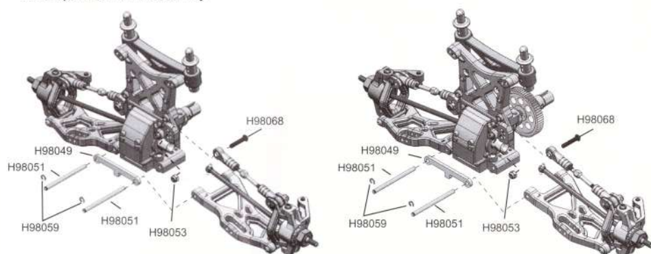
8. Suspension Arm Assembly
